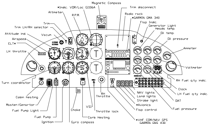
Fig. 7-2. INSTRUMENT PANEL
