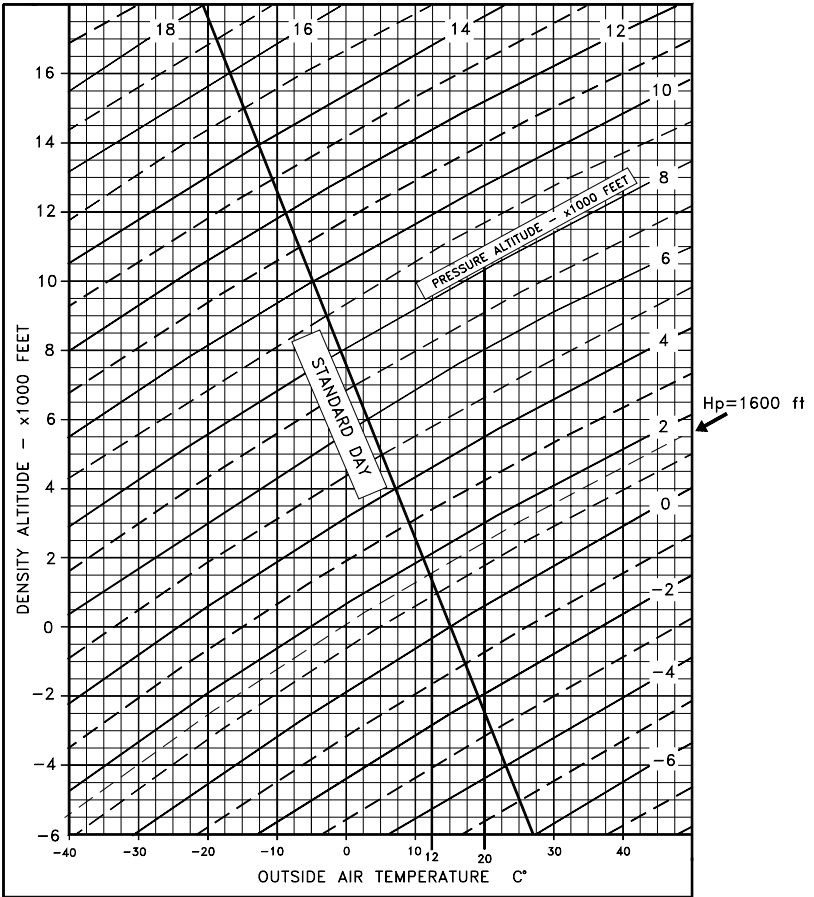
Fig.5-2. ICAO CHART
