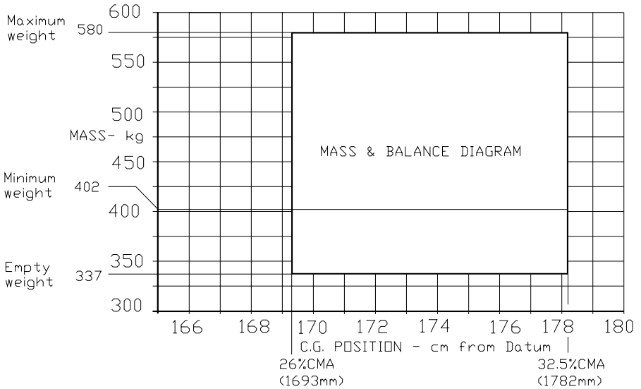
Fig 6-3 C.G. RANGE CHART
